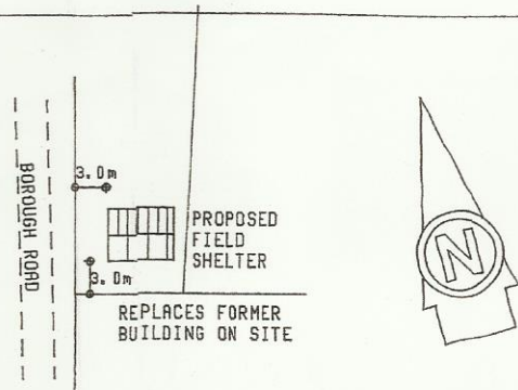
SITE PLAN [part] 1:500
