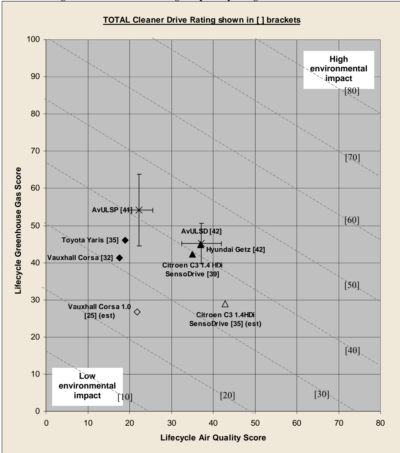
Figure 9.2 Cleaner Drive Rating for specific passenger cars - SUPERMINI
