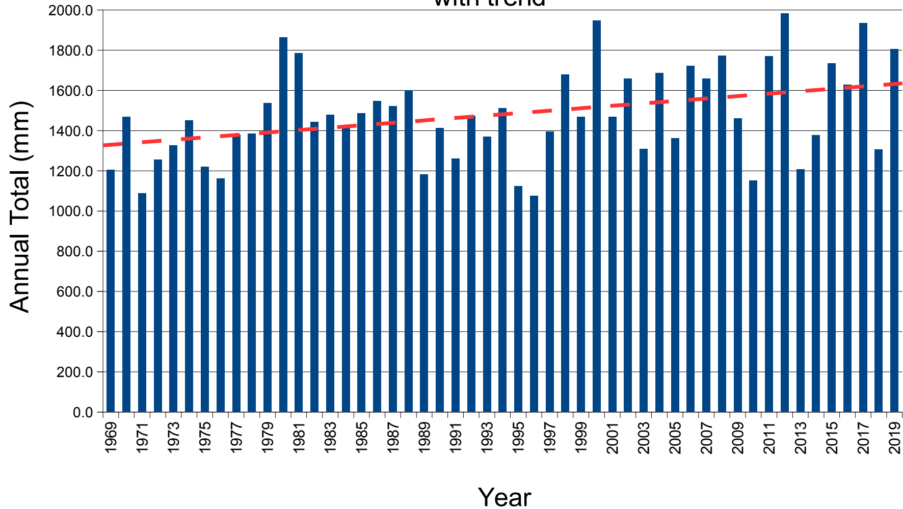
Chipping Annual Rainfall 1969-2019 with trend
